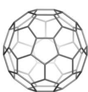
C_{60}
