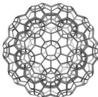
C_{60}(D_{O60})_{-750}
