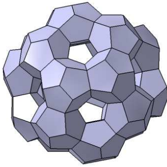
C_{60}
