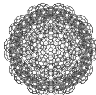
TR(DU(C_{60}(D_{O60})_{750})_{662})_{-5040}
